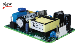
OPS2x3-40 76.2(L) X 50.8(W) x 30(H)mm
