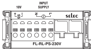
Figure 4.1 : FL-RL-PS-230V wiring
