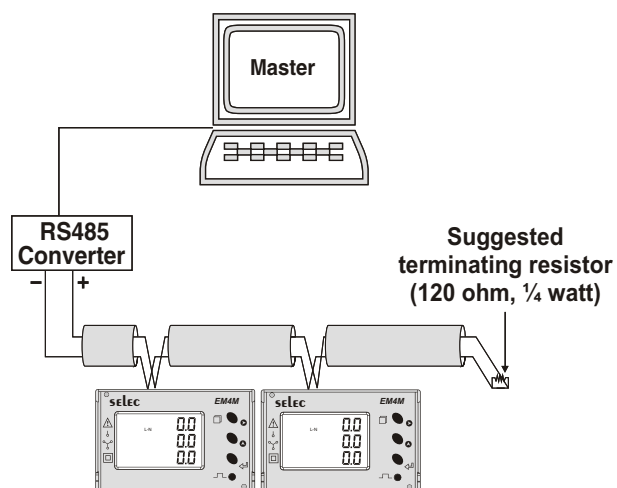
CONNECTION DIAGRAM FOR COMMUNICATION
