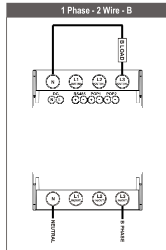
1 Phase - 2 Wire - B
