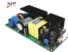
OPS2x4-60 101.6(L) X 50.8(W) x 30(H)mm
