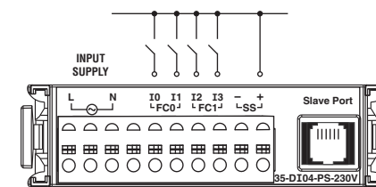
Figure 5.2 : Digital Inputs using internal 10V power supply
