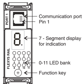
Figure 3.1 FL-RL-LG-X-X-X Display
